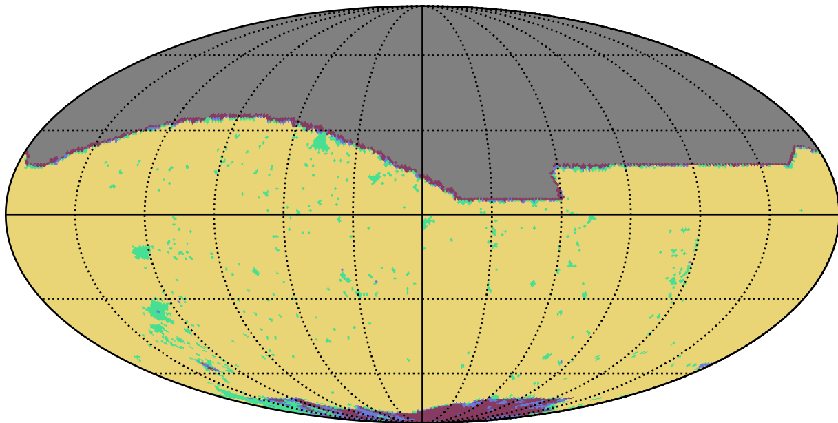
weather_cloudso2v3.4_10yrs r band: YearCoverage night
