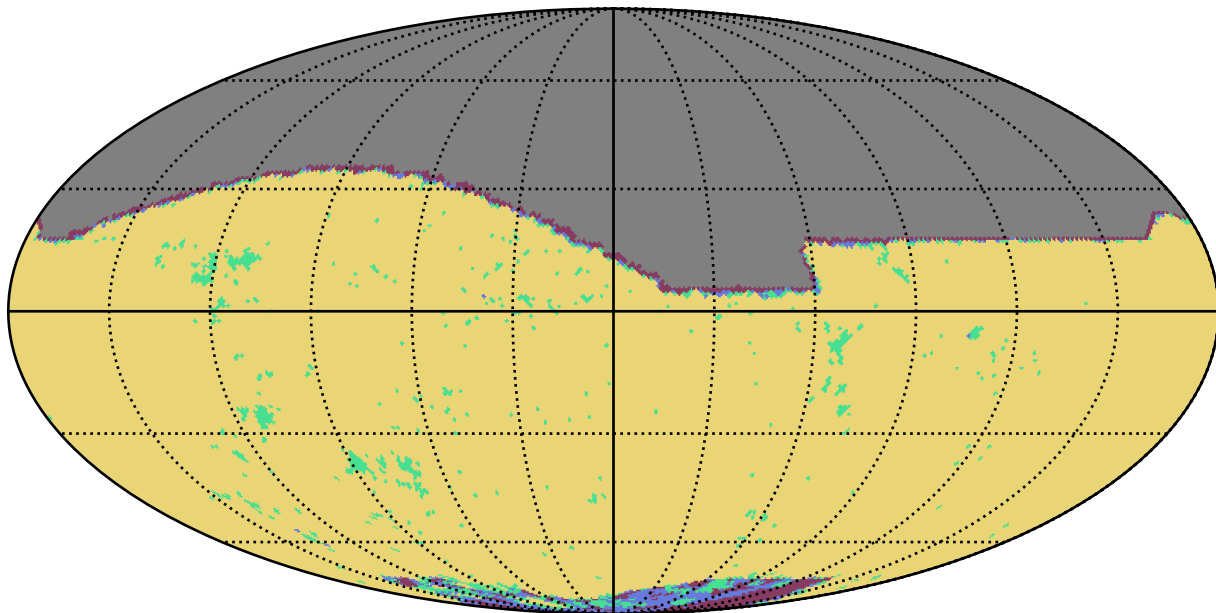
weather_cloudso2v3.4_10yrs i band: YearCoverage night
