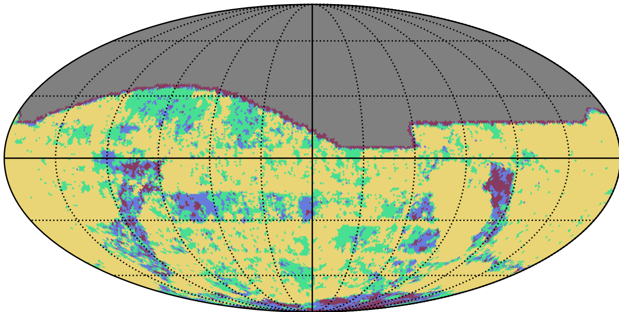
weather_cloudso2v3.4_10yrs g band: YearCoverage night
