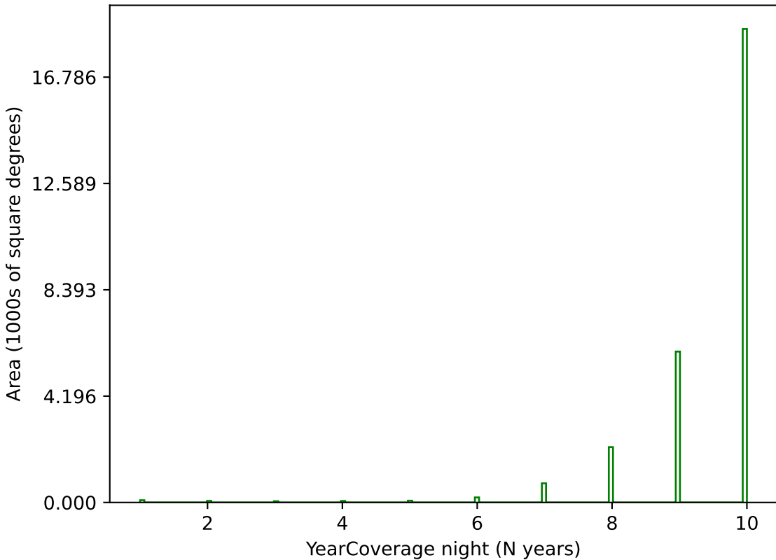
weather_cloudso2v3.4_10yrs g band: YearCoverage night
