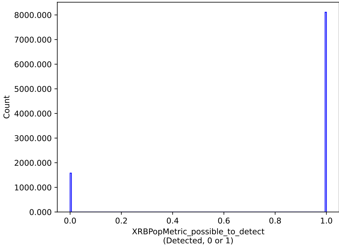
weather_cloudso2v3.4_10yrs : XRBPoMetric_possible_to_detect
