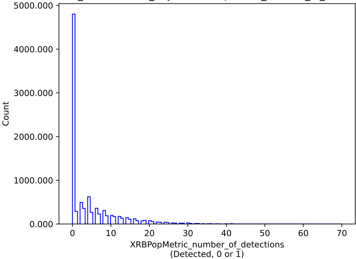
weather_cloudso2v3.4_10yrs : XRBPoMetric_number_of_detections
