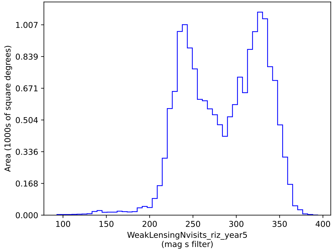
weather_cloudso2v3.4_10yrs gri band non-DD: WeakLensingNvisits_riz_year5
