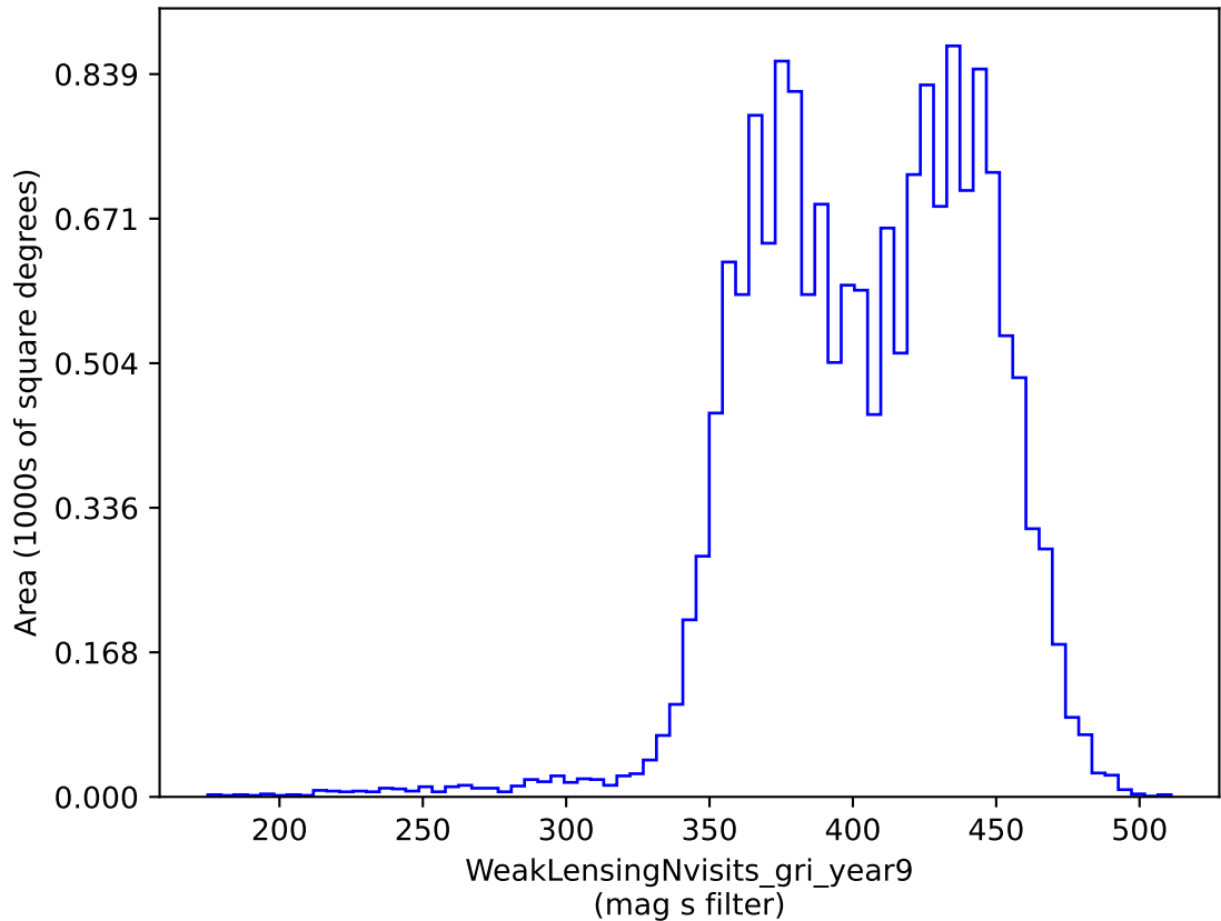
weather_cloudso2v3.4_10yrs gri band non-DD: WeakLensingNvisits_gri_year9
