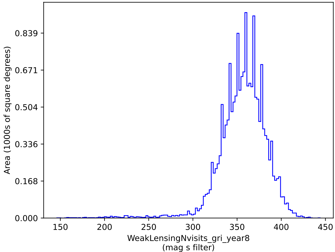
weather_cloudso2v3.4_10yrs gri band non-DD: WeakLensingNvisits_gri_year8
