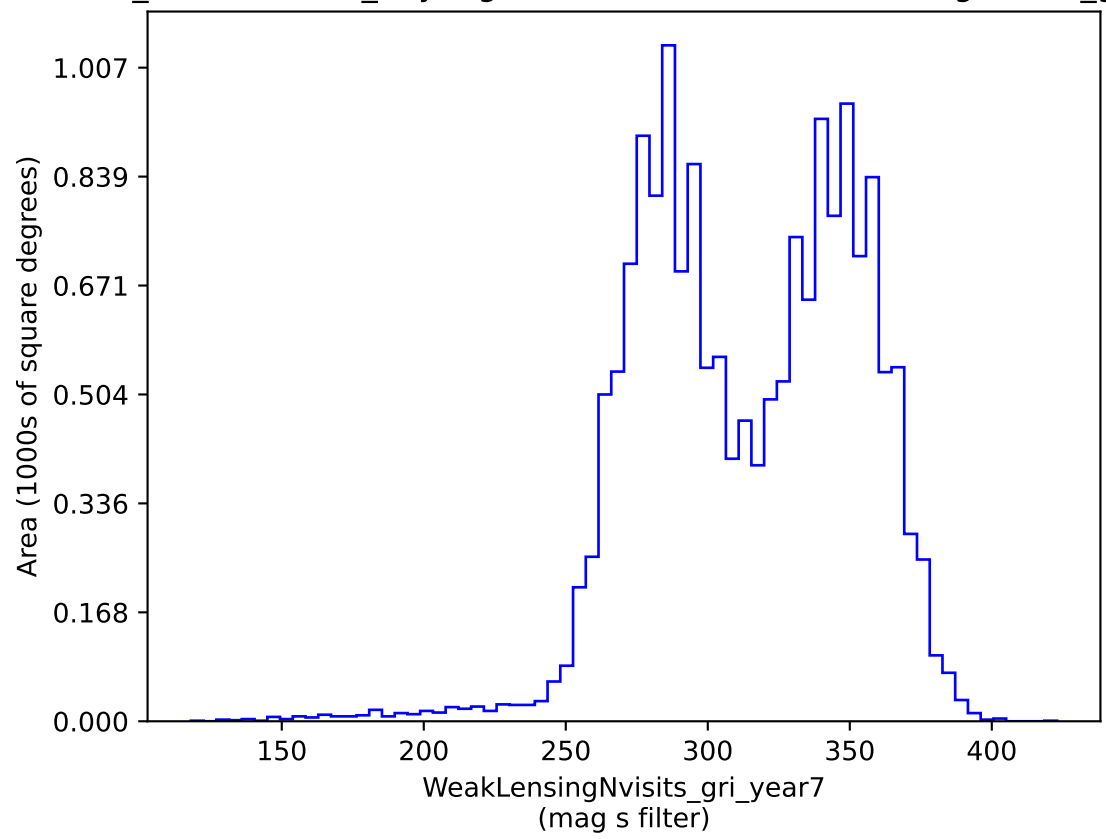
weather_cloudso2v3.4_10yrs gri band non-DD: WeakLensingNvisits_gri_year7
