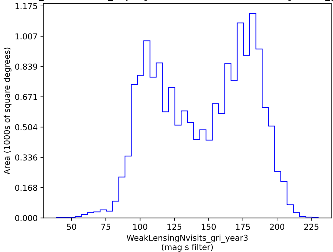
weather_cloudso2v3.4_10yrs gri band non-DD: WeakLensingNvisits_gri_year3
