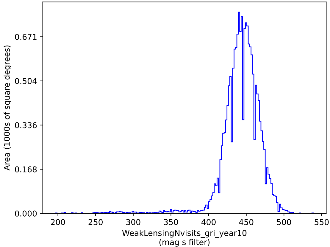
weather_cloudso2v3.4_10yrs gri band non-DD: WeakLensingNvisits_gri_year10
