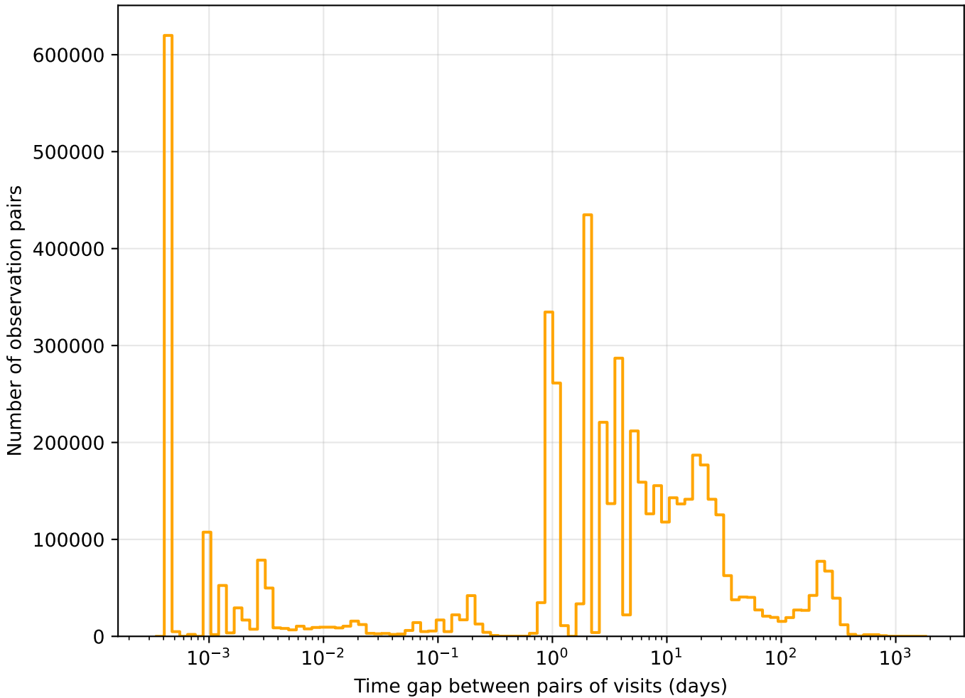
weather_cloudso2v3.4_10yrs r band: Tgaps observationStartMJD
