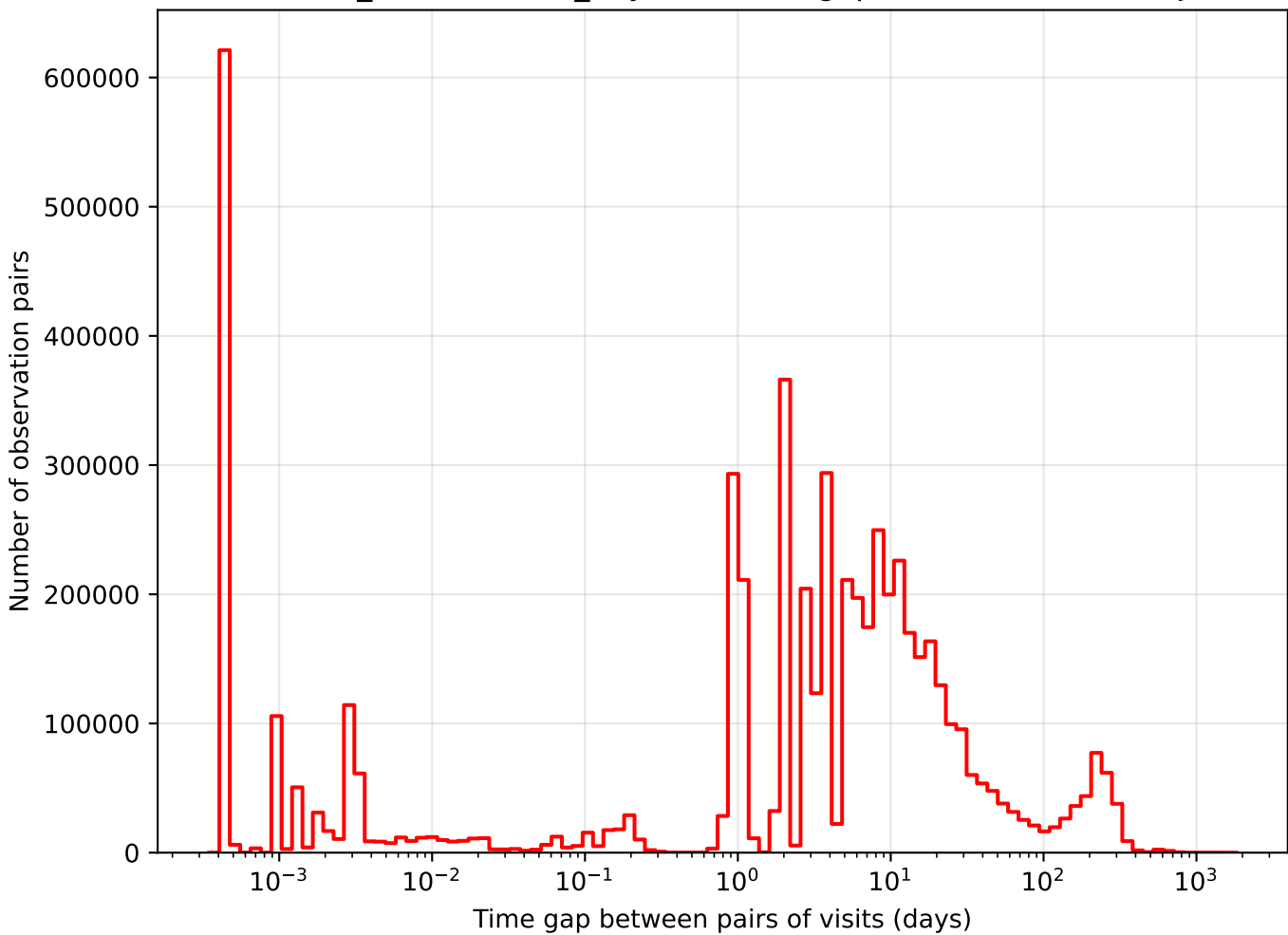
weather_cloudso2v3.4_10yrs i band: Tgaps observationStartMJD
