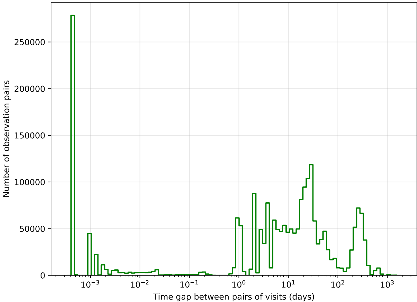
weather_cloudso2v3.4_10yrs g band: Tgaps observationStartMJD
