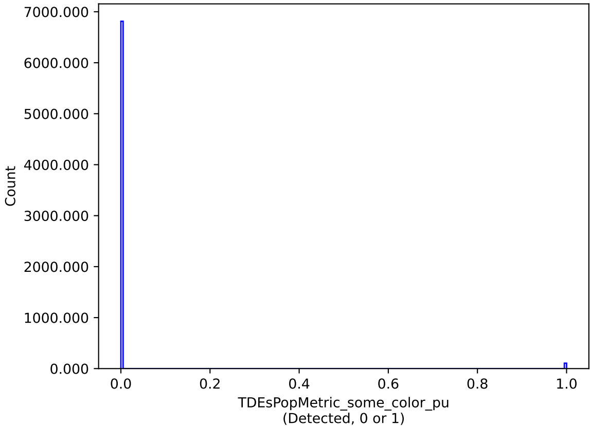
weather_cloudso2v3.4_10yrs : TDEsPopMetric_some_color_pu
