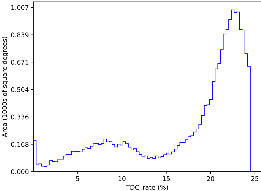
weather_cloudso2v3.4_10yrs : TDC_rate
