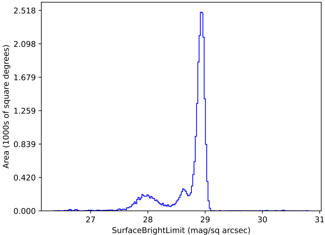
weather_cloudso2v3.4_10yrs u: SurfaceBrightLimit
