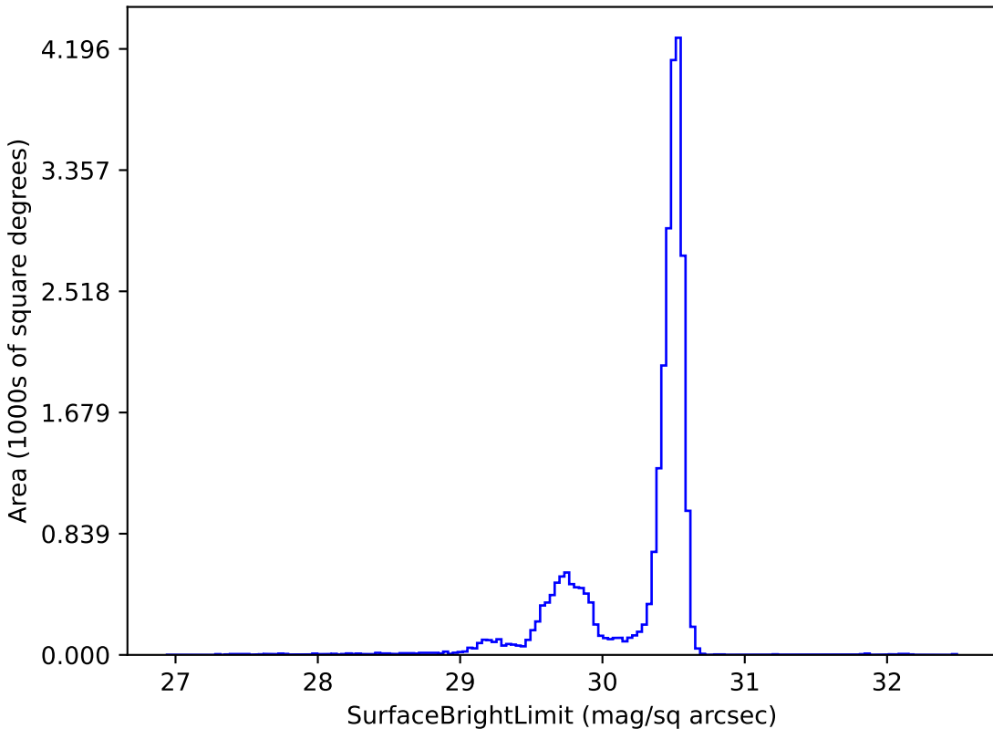
weather_cloudso2v3.4_10yrs r: SurfaceBrightLimit
