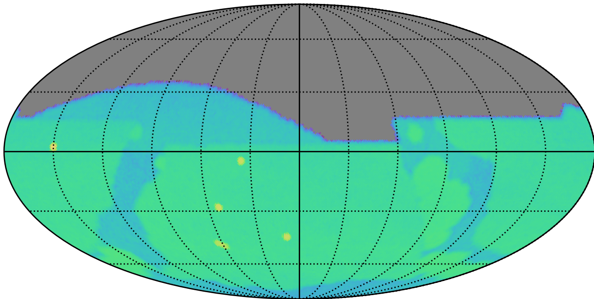
weather_cloudso2v3.4_10yrs g: SurfaceBrightLimit
