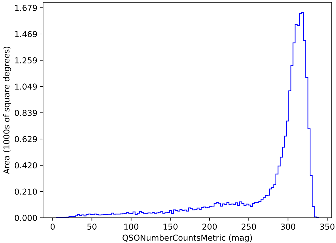
weather_cloudso2v3.4_10yrs u band and non-DD: QSONumberCountsMetric
