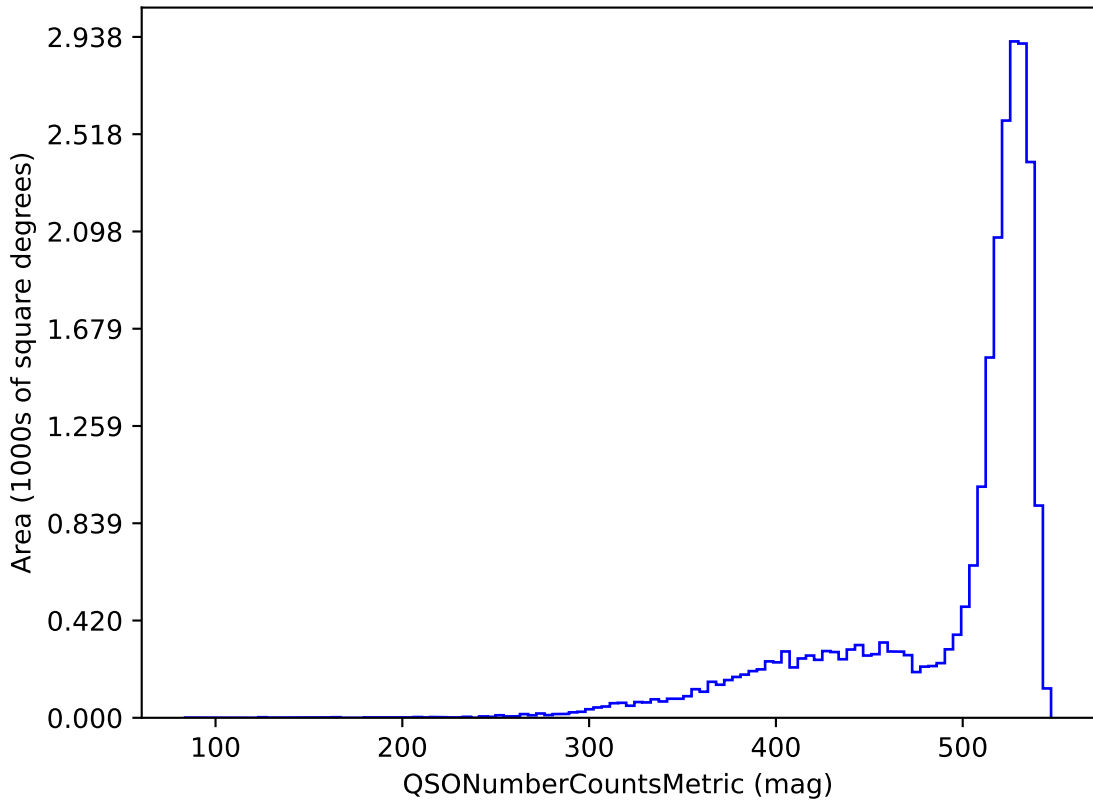
weather_cloudso2v3.4_10yrs r band and non-DD: QSONumberCountsMetric
