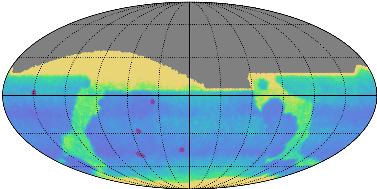
weather_cloudso2v3.4_10yrs : Proper Motion Uncert @ 24.0
