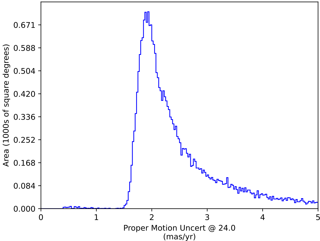
weather_cloudso2v3.4_10yrs : Proper Motion Uncert @ 24.0
