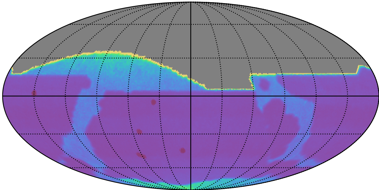
weather_cloudso2v3.4_10yrs : Proper Motion Uncert @ 20.5
