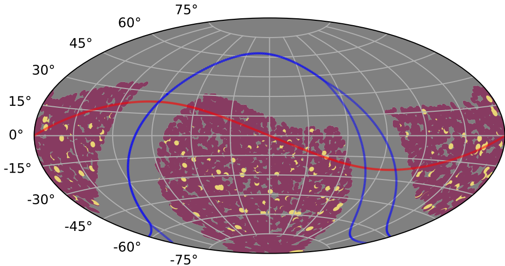
weather_cloudso2v3.4_10yrs : PrestoKNe_score_s
