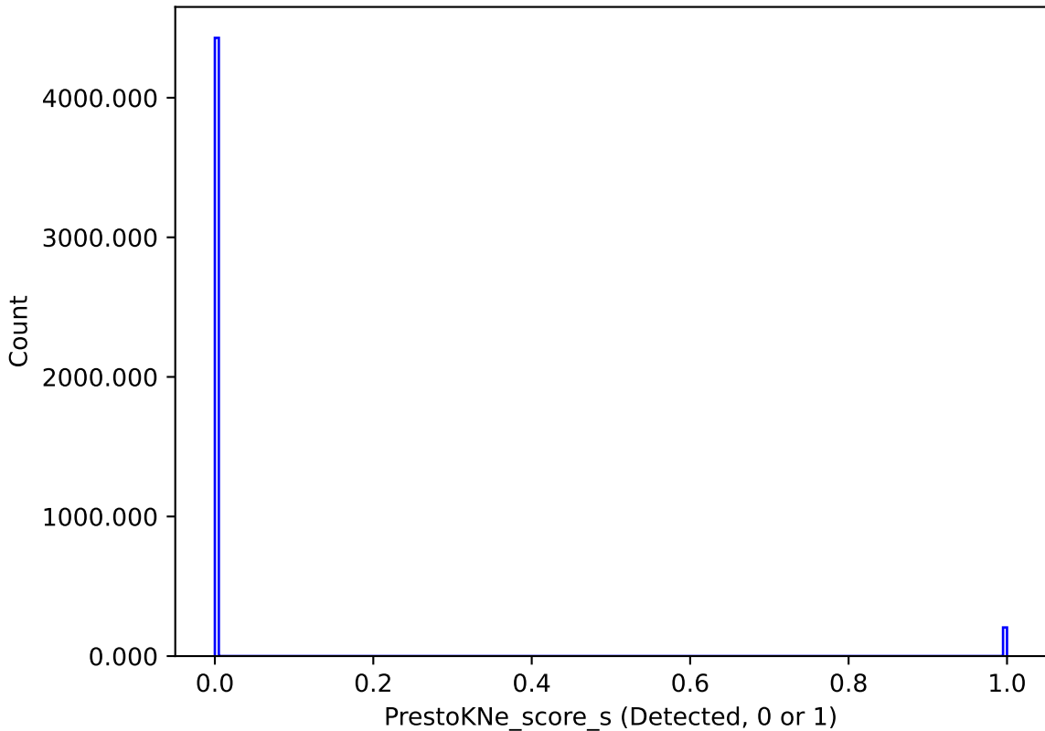
weather_cloudso2v3.4_10yrs : PrestoKNe_score_s
