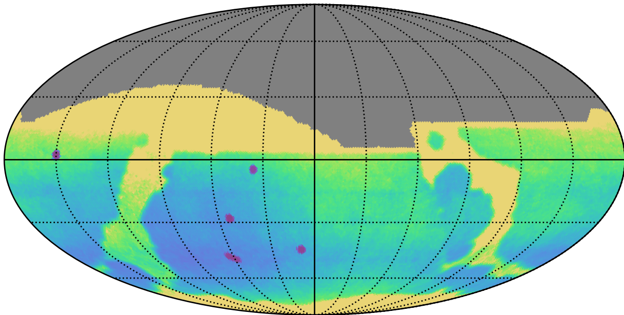
weather_cloudso2v3.4_10yrs : Parallax Uncert @ 24.0
