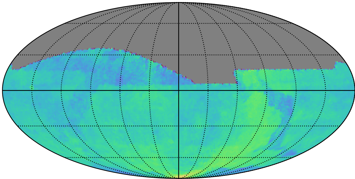
weather_cloudso2v3.4_10yrs : Parallax Coverage @ 24.0
