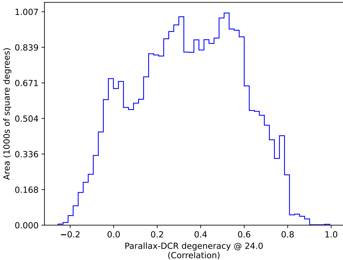
weather_cloudso2v3.4_10yrs : Parallax-DCR degeneracy @ 24.0
