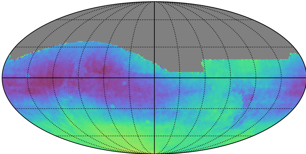
weather_cloudso2v3.4_10yrs : Parallax-DCR degeneracy @ 22.4
