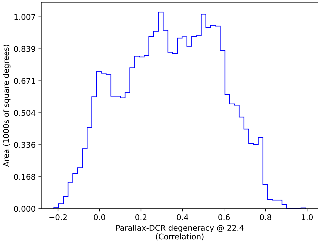
weather_cloudso2v3.4_10yrs : Parallax-DCR degeneracy @ 22.4
