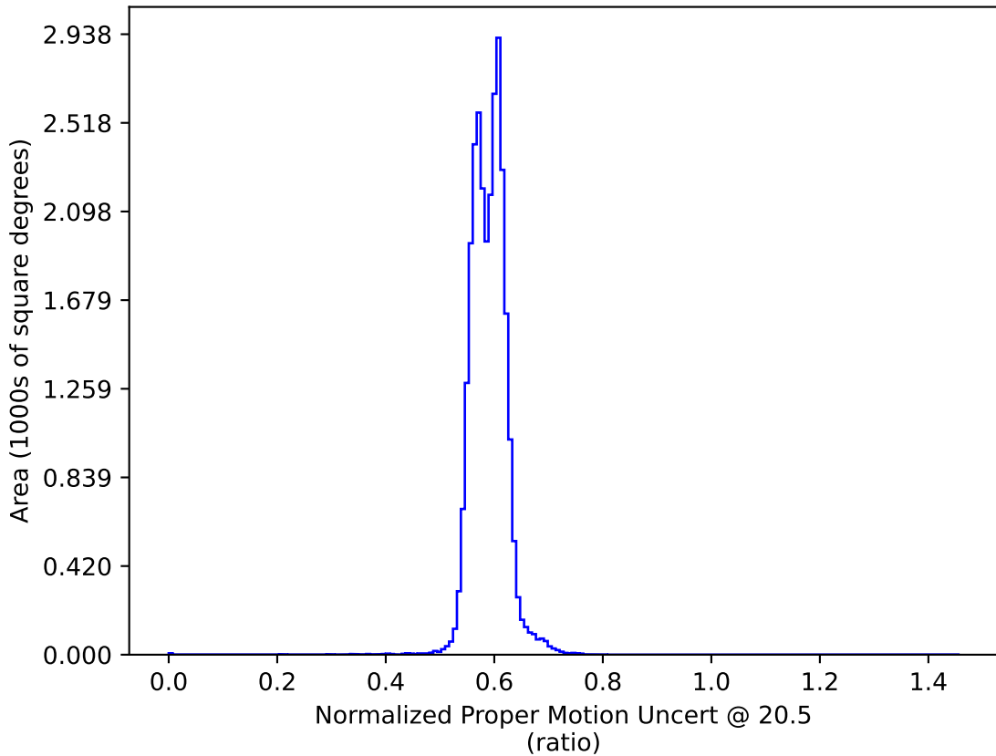
weather_cloudso2v3.4_10yrs : Normalized Proper Motion Uncert @ 20.5
