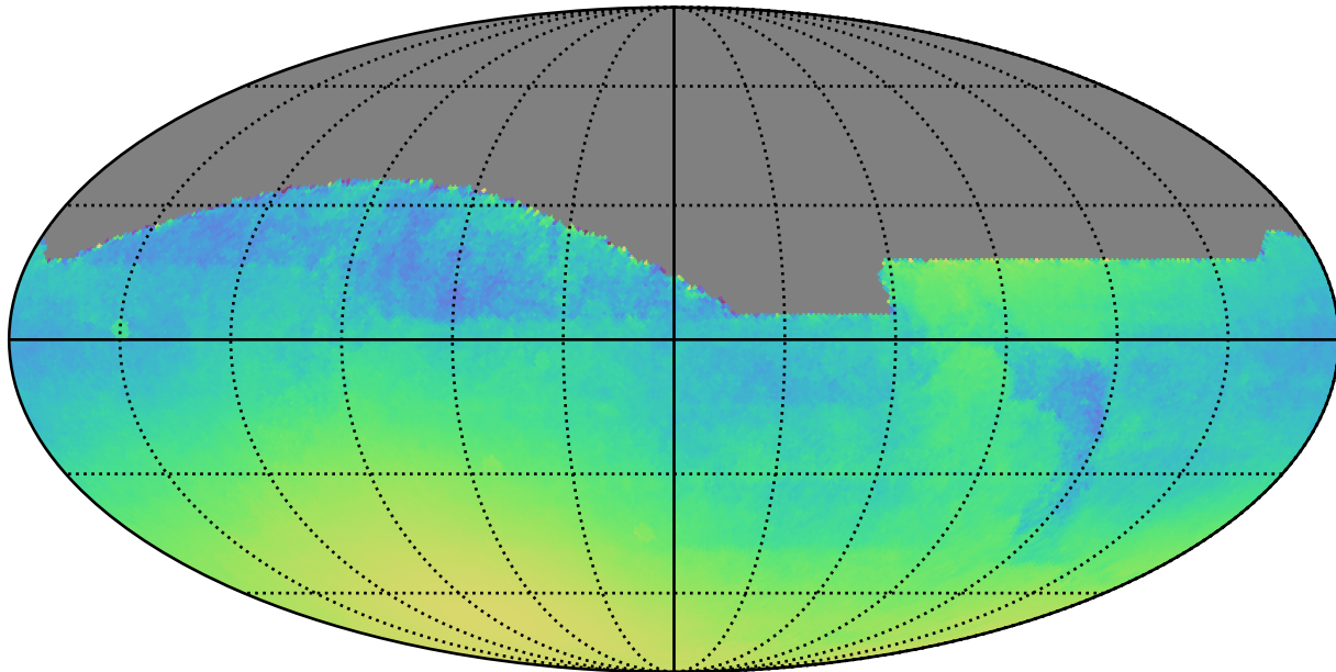
weather_cloudso2v3.4_10yrs : Normalized Parallax Uncert @ 24.0
