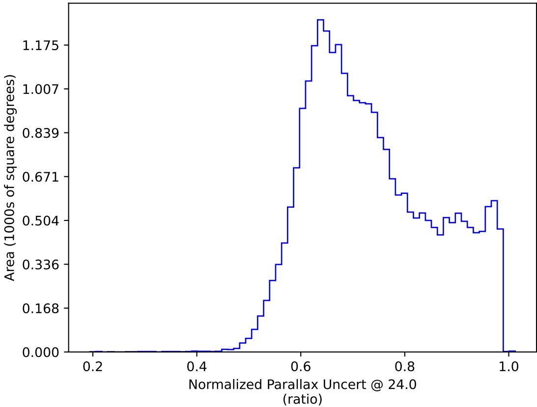
weather_cloudso2v3.4_10yrs : Normalized Parallax Uncert @ 24.0
