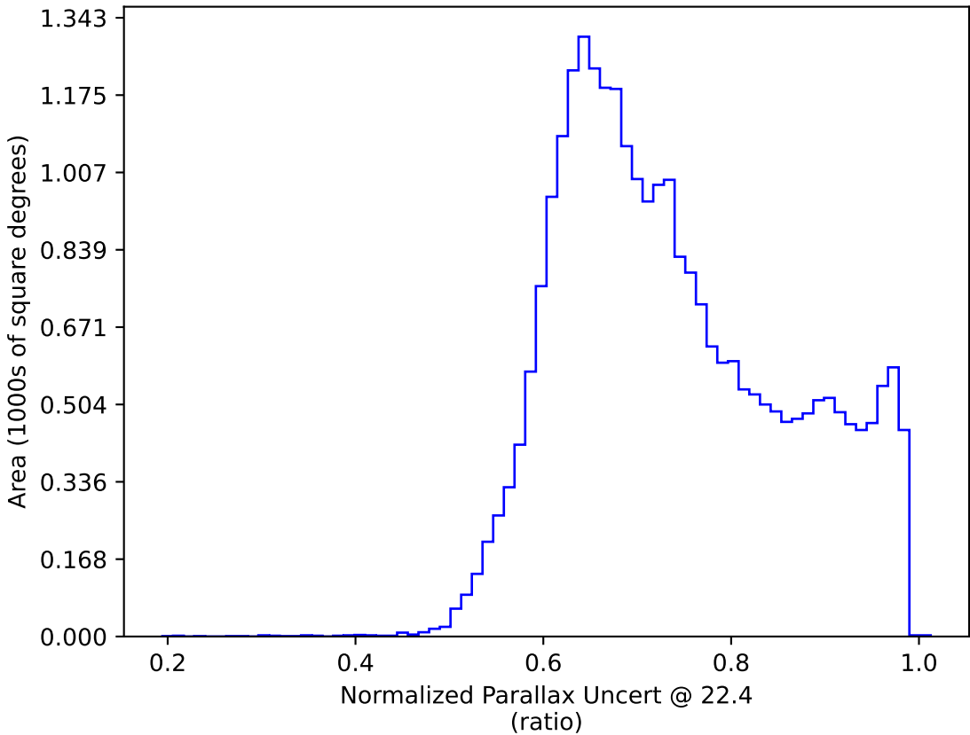
weather_cloudso2v3.4_10yrs : Normalized Parallax Uncert @ 22.4
