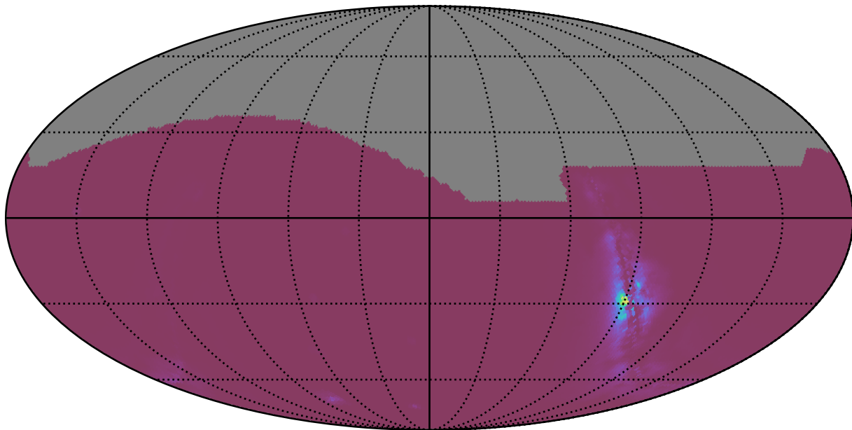
weather_cloudso2v3.4_10yrs : NlcPoints
