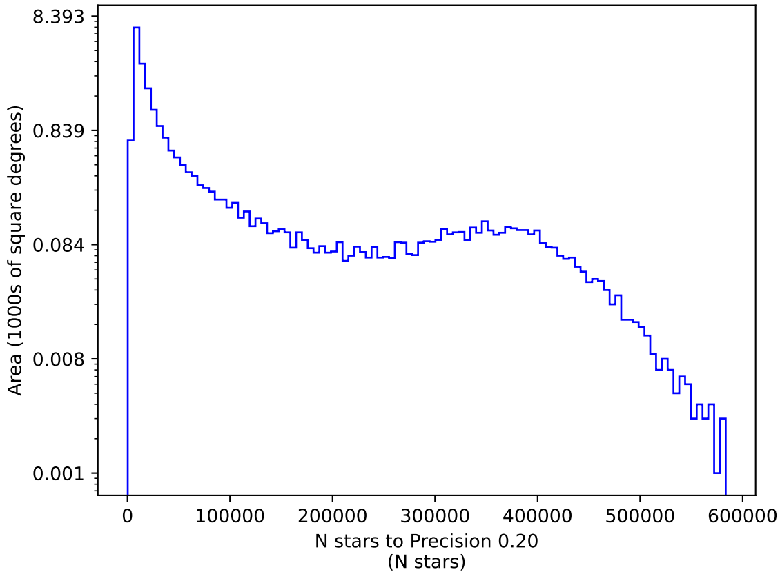
weather_cloudso2v3.4_10yrs y: N stars to Precision 0.20
