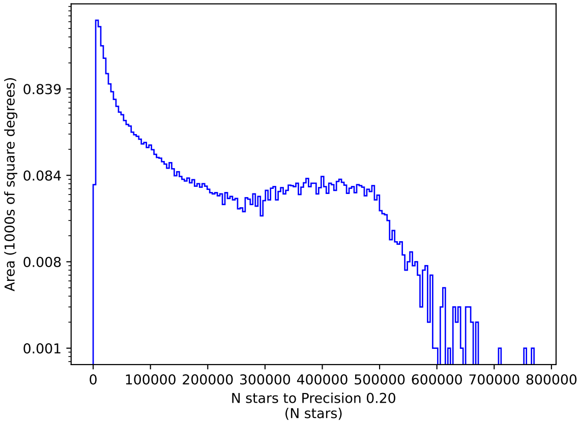
weather_cloudso2v3.4_10yrs r: N stars to Precision 0.20
