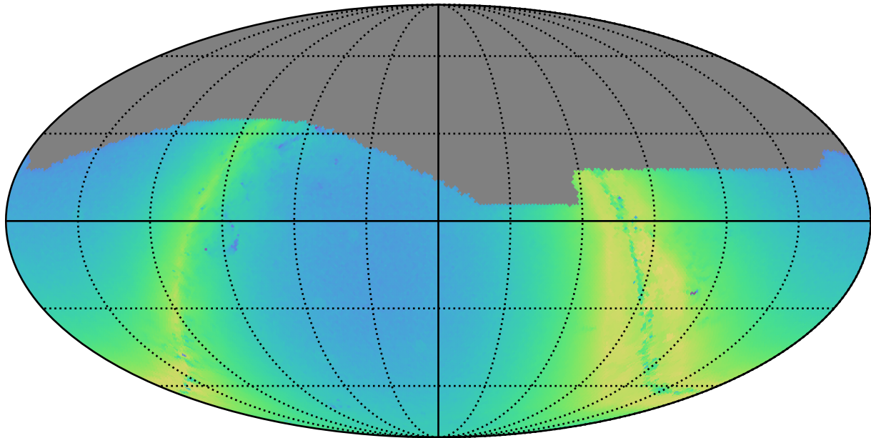
weather_cloudso2v3.4_10yrs g: N stars to Precision 0.20
