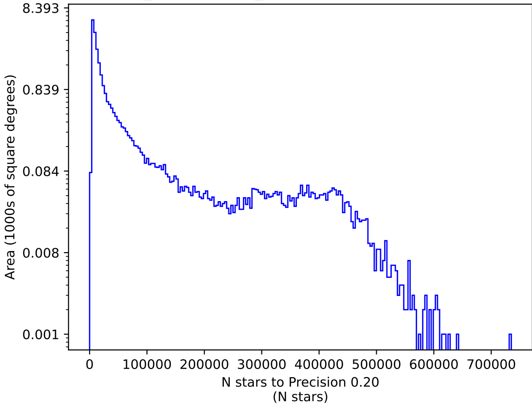
weather_cloudso2v3.4_10yrs g: N stars to Precision 0.20
