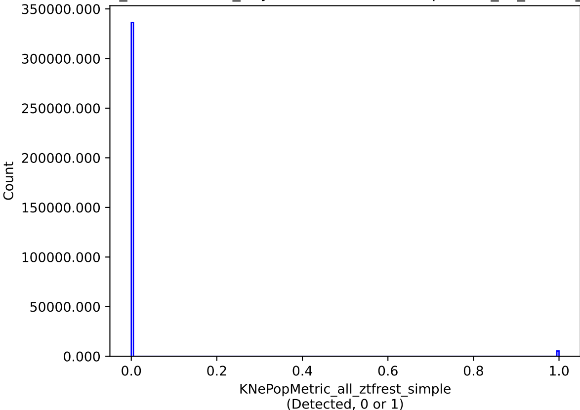
weather_cloudso2v3.4_10yrs all models: KNePopMetric_all_ztfrest_simple
