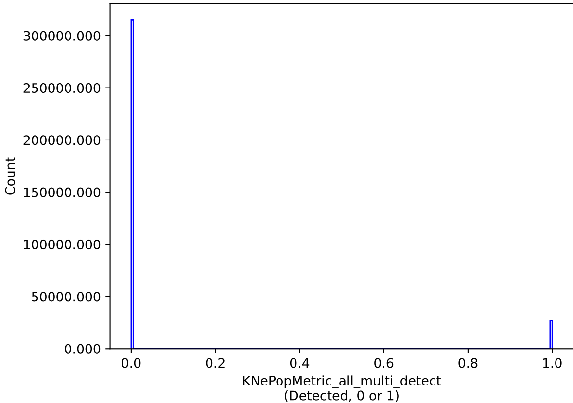
weather_cloudso2v3.4_10yrs all models: KNePopMetric_all_multi_detect
