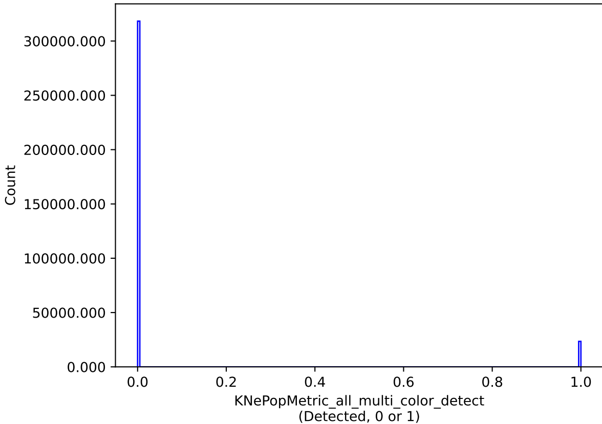
weather_cloudso2v3.4_10yrs all models: KNePopMetric_all_multi_color_detect
