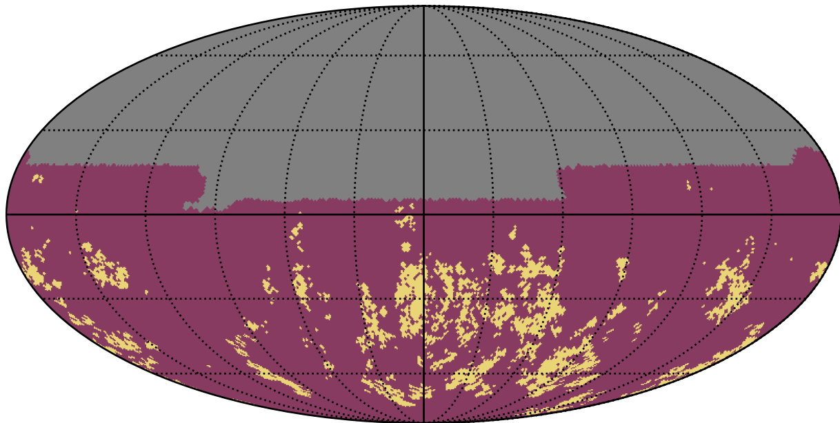
weather_cloudso2v3.4_10yrs u band: Gaps_7hr
