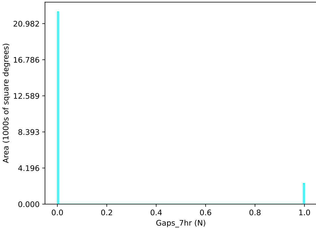
weather_cloudso2v3.4_10yrs u band: Gaps_7hr
