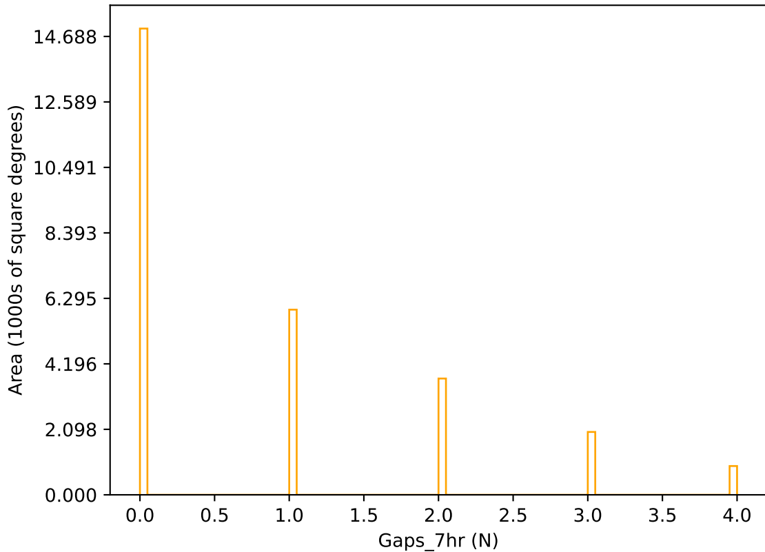
weather_cloudso2v3.4_10yrs r band: Gaps_7hr
