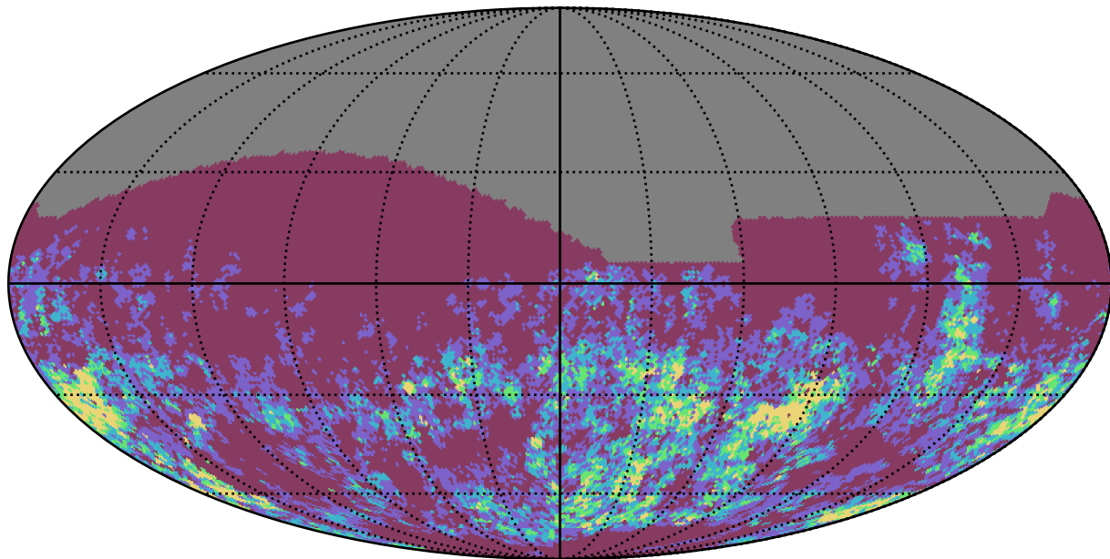
weather_cloudso2v3.4_10yrs i band: Gaps_7hr
