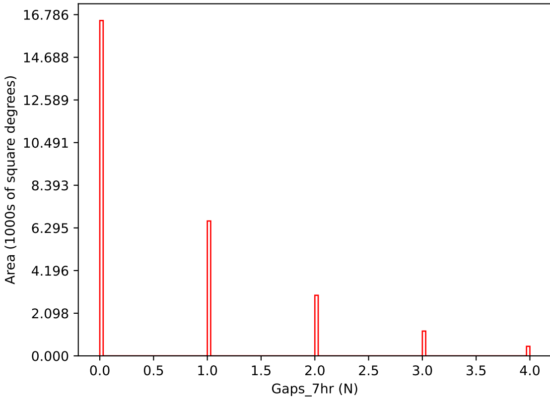
weather_cloudso2v3.4_10yrs i band: Gaps_7hr
