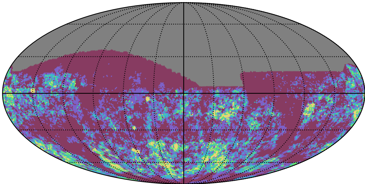
weather_cloudso2v3.4_10yrs z band: Gaps_3hr
